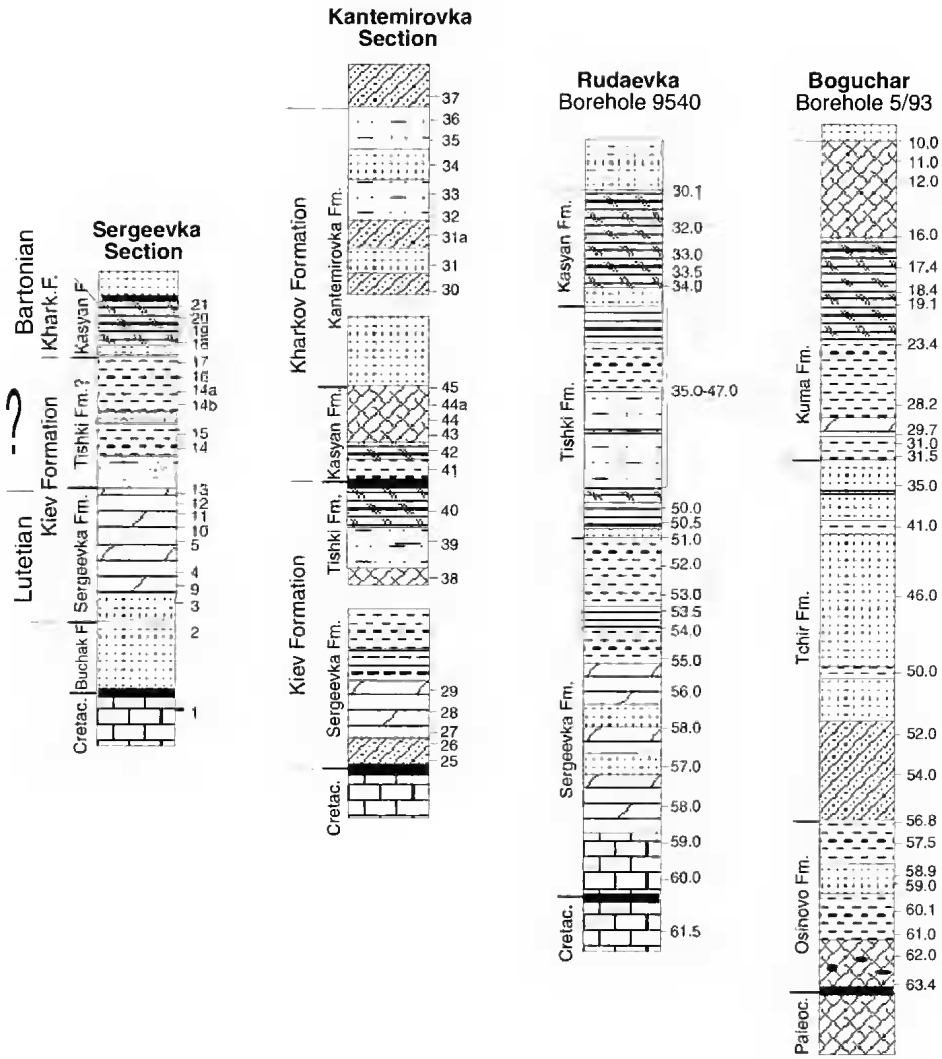
Fig. 2. — A, correlation of studied sections of the eastern slope of the Dnieper-Donets Depression. N 1-2 , nannofossil assemblage; F, foraminifera assemblage; R 1-5 , radiolaria assemblage; D 1-2 , diatoms assemblage. B, samples number from the sections.
